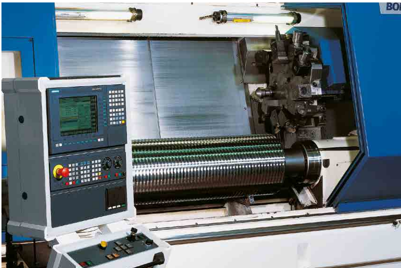
Advanced CNC lathes are used to turn the rope drums in one operation, an approach that ensures perfectly smooth running of the rope drums during operation.
