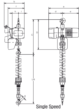
Single Speed
